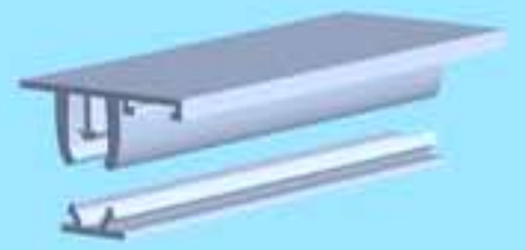
Double lisse Ghost invisible plafond / Double Ghost Rail for ceiling anchorage
